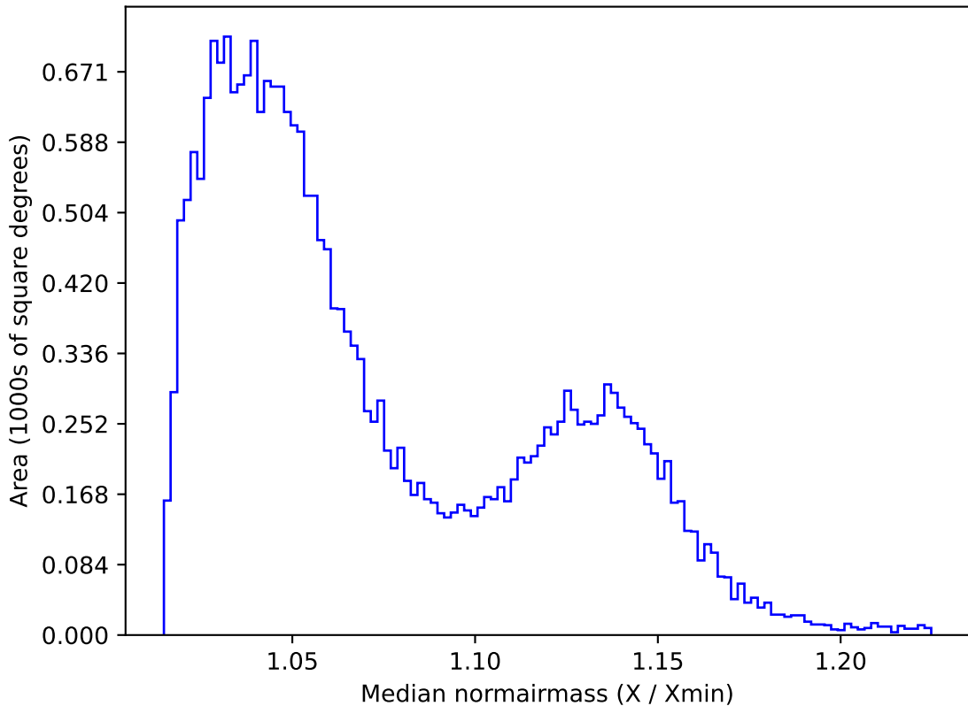
ddf_acor_sf10_lsf40_lsr10_v3.4_10yrs All sky i band: Median normairmass
