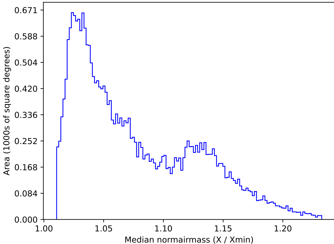
ddf_acor_sf10_lsf40_lsr10_v3.4_10yrs All sky g band: Median normairmass
