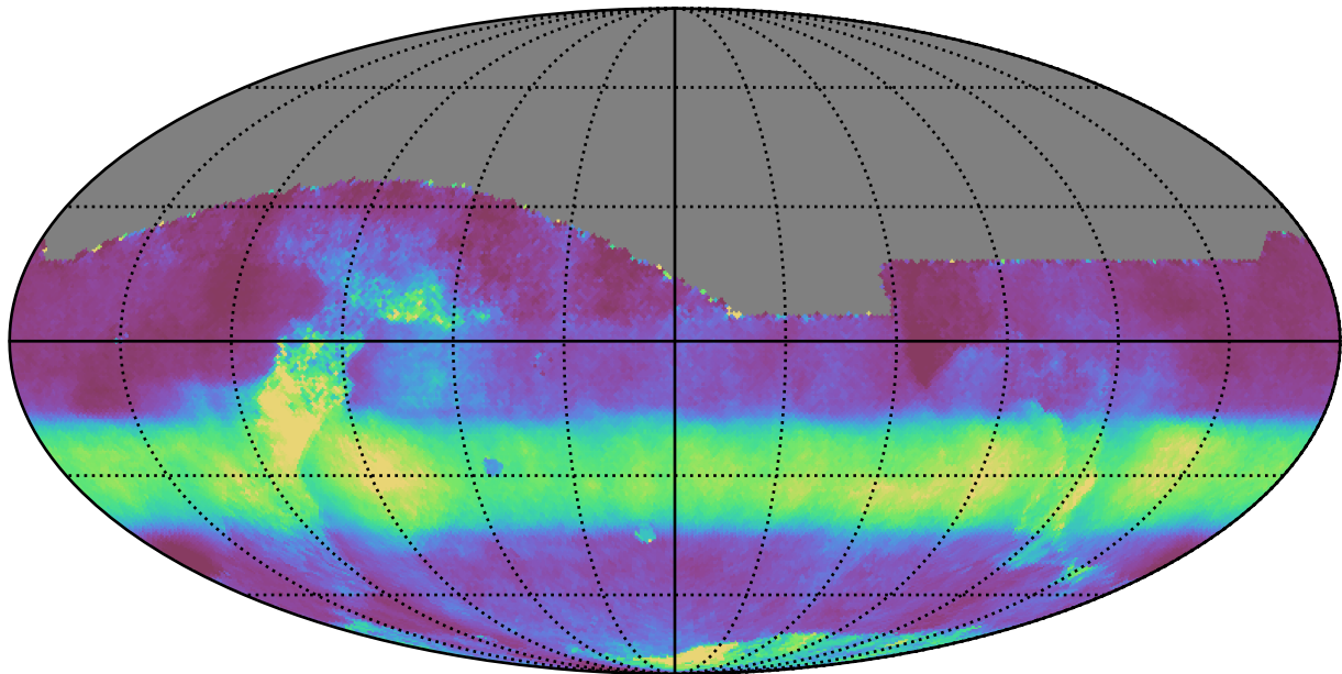
ddf_acor_sf10_lsf40_lsr10_v3.4_10yrs All sky all bands: Median normairmass
