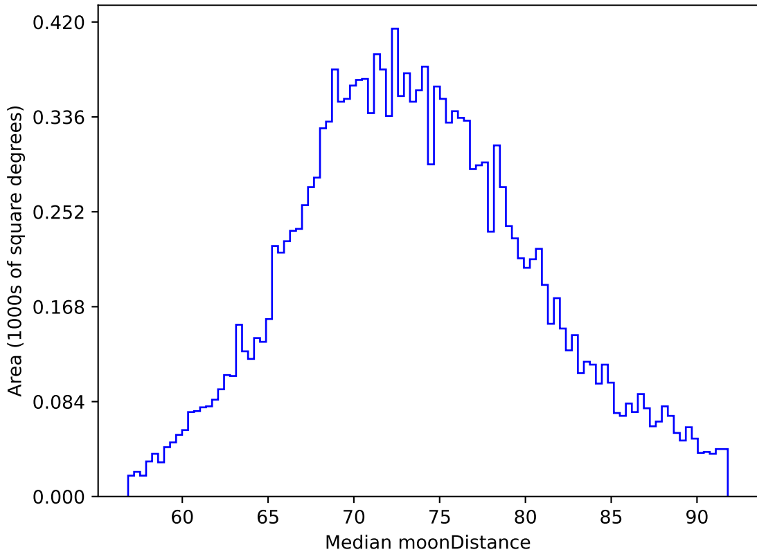
ddf_acor_sf10_lsf40_lsr10_v3.4_10yrs WFD z band: Median moonDistance
