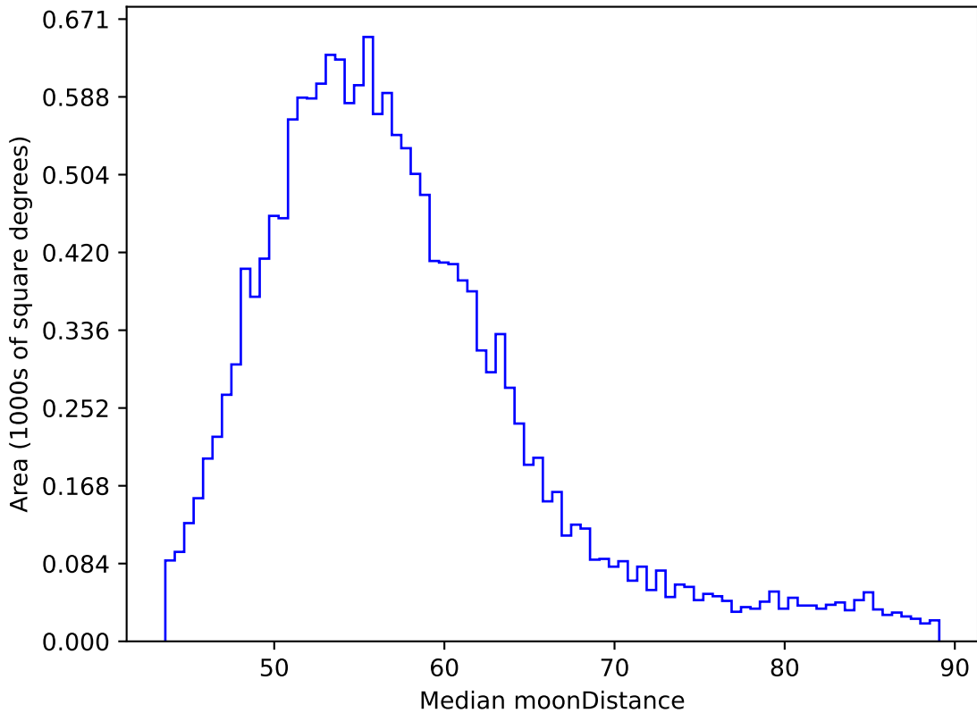
ddf_acor_sf10_lsf40_lsr10_v3.4_10yrs WFD y band: Median moonDistance
