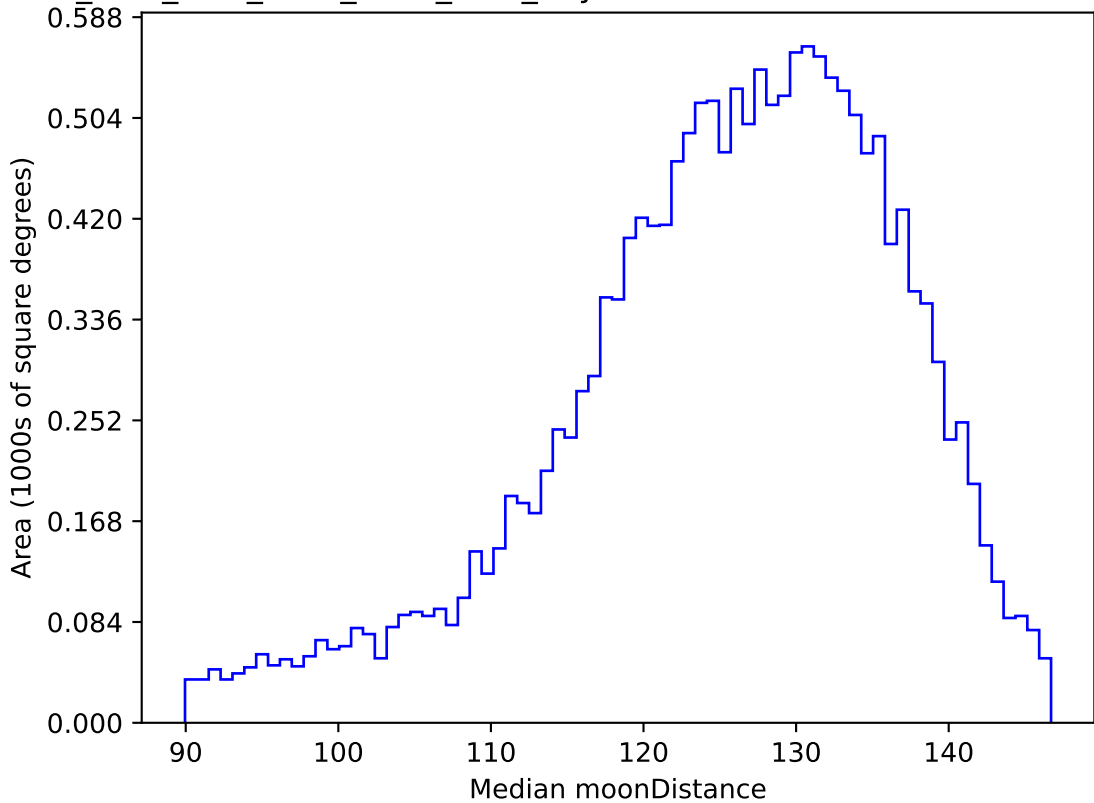
ddf_acor_sf10_lsf40_lsr10_v3.4_10yrs WFD u band: Median moonDistance
