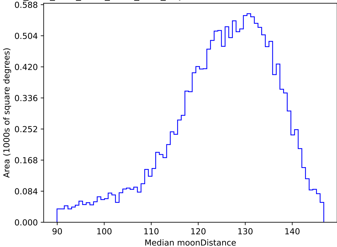
ddf_acor_sf10_ls40_lsr10_v3.4_10yrs WFD u band: Median moonDistance
