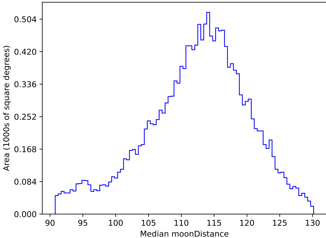
ddf_acor_sf10_lsf40_lsr10_v3.4_10yrs WFD r band: Median moonDistance
