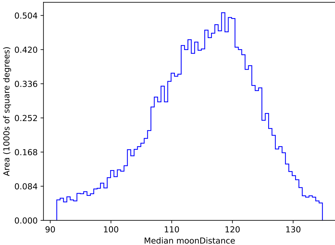
ddf_acor_sf10_lsf40_lsr10_v3.4_10yrs WFD g band: Median moonDistance
