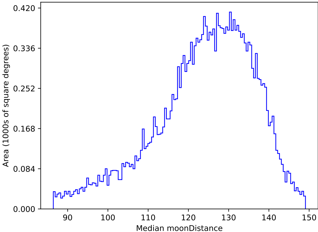
ddf_acor_sf10_lsf40_lsr10_v3.4_10yrs All sky u band: Median moonDistance
