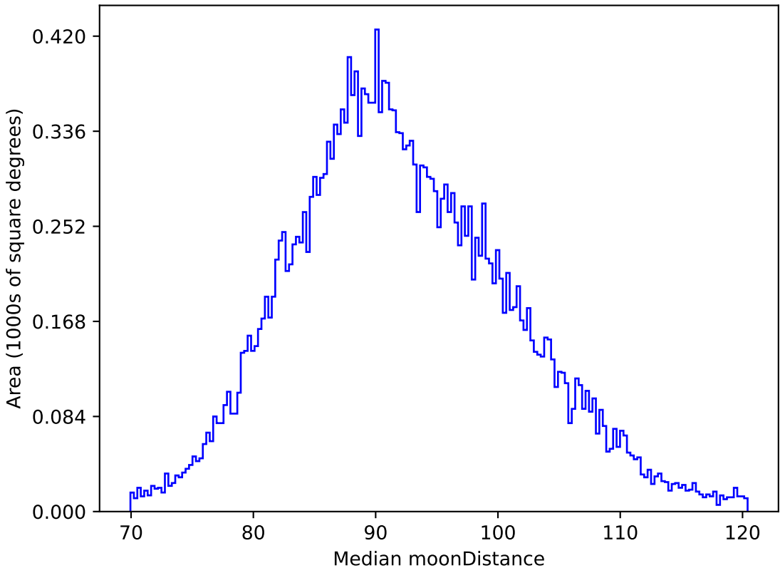
ddf_acor_sf10_lsf40_lsr10_v3.4_10yrs All sky i band: Median moonDistance
