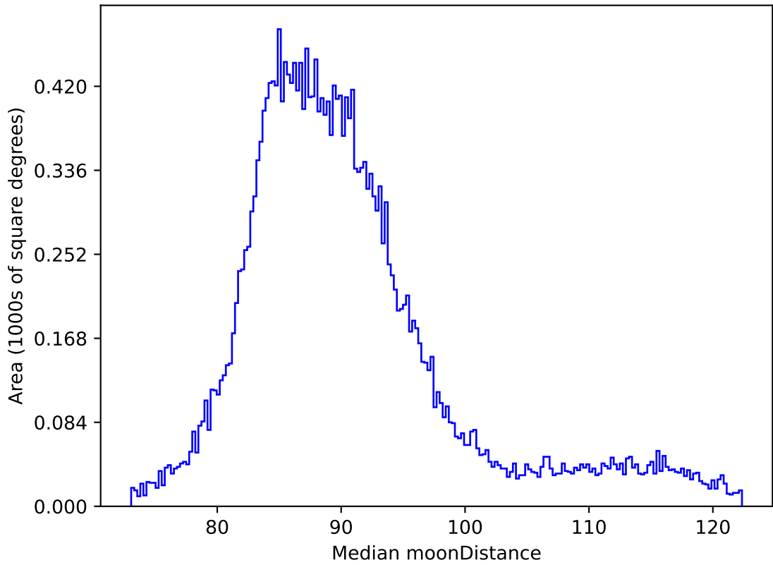
ddf_acor_sf10_lsf40_lsr10_v3.4_10yrs All sky all bands: Median moonDistance
