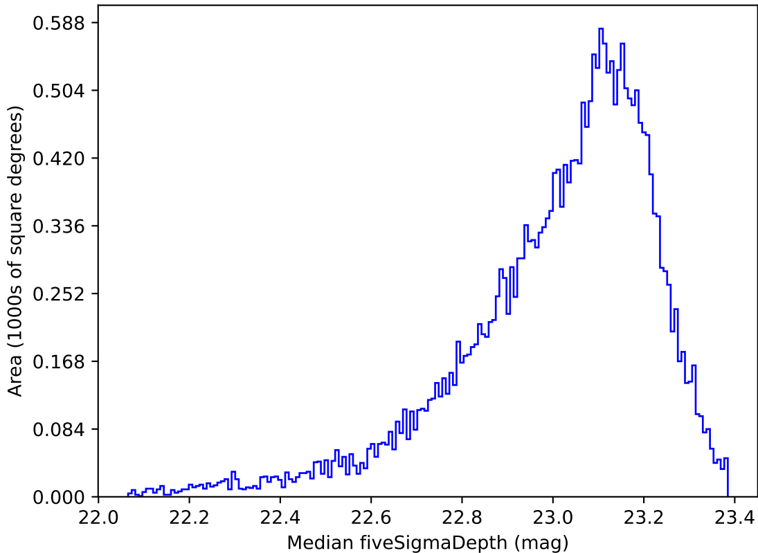
ddf_acor_sf10_lsf40_lsr10_v3.4_10yrs Yr 1 z band: Median fiveSigmaDepth
