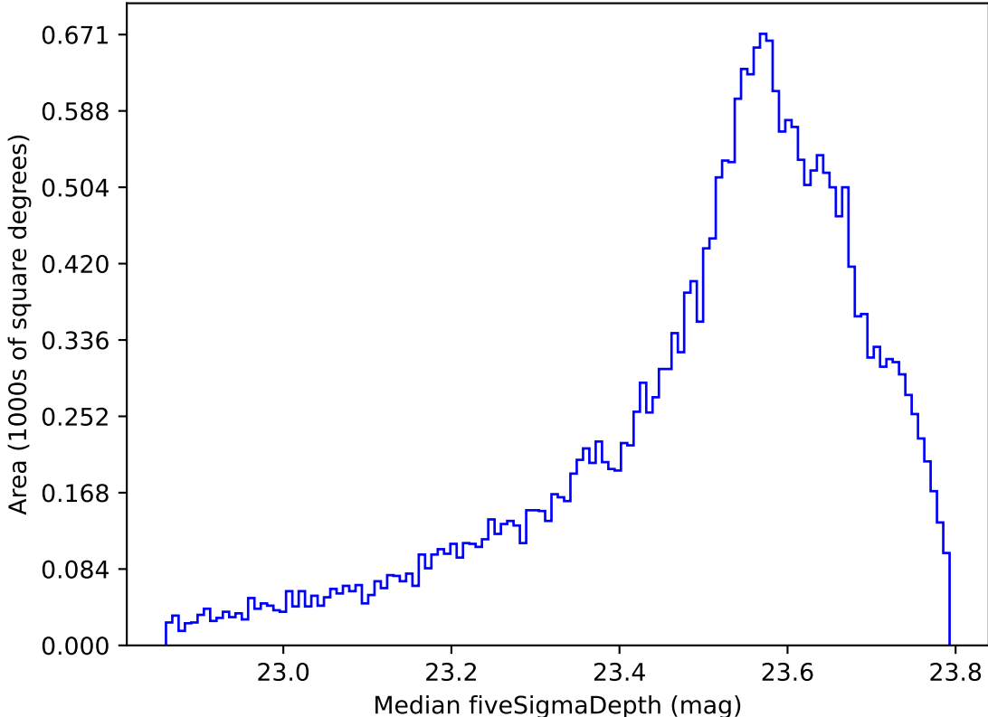
ddf_acor_sf10_lsf40_lsr10_v3.4_10yrs All sky i band: Median fiveSigmaDepth
