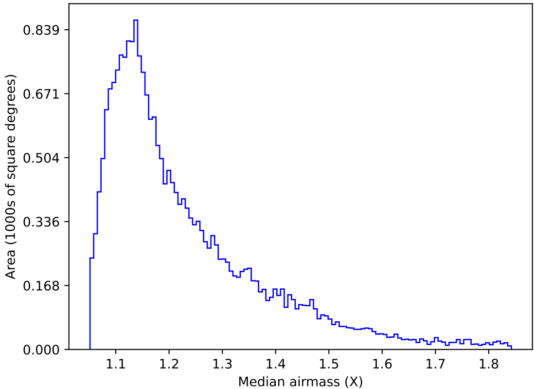
ddf_acor_sf10_lsf40_lsr10_v3.4_10yrs Yr 1 u band: Median airmass
