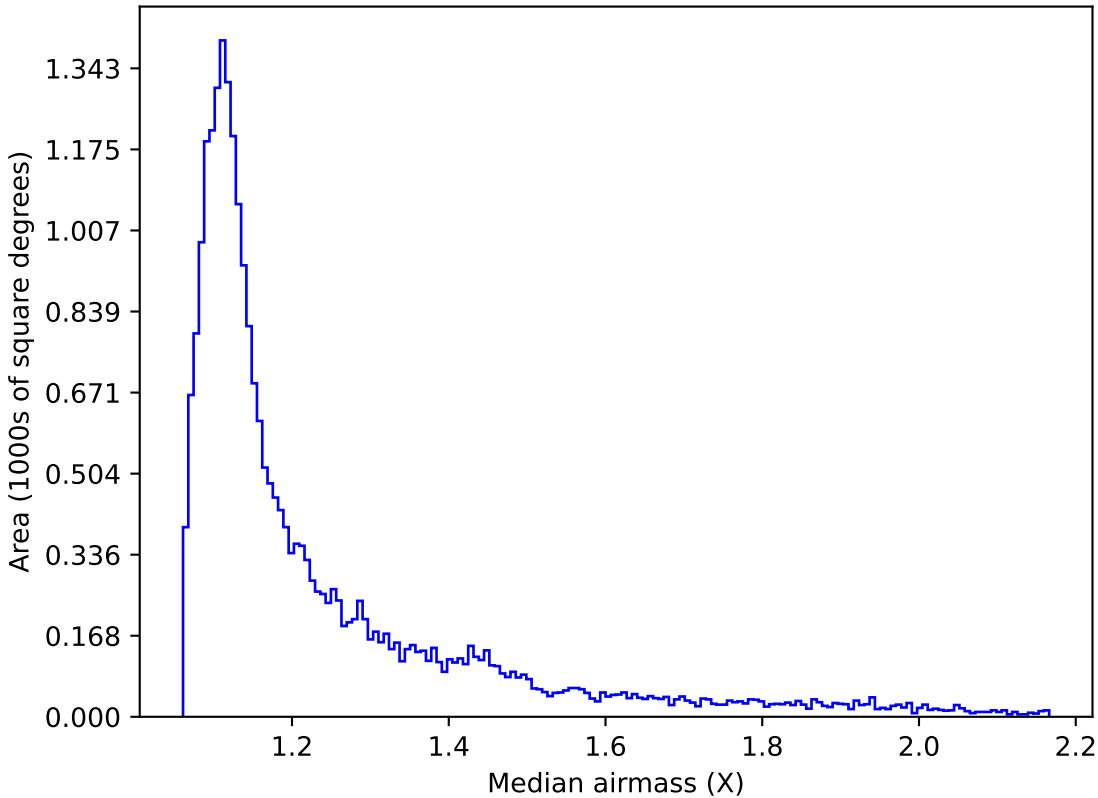
ddf_acor_sf10_lsf40_lsr10_v3.4_10yrs Yr 1 i band: Median airmass
