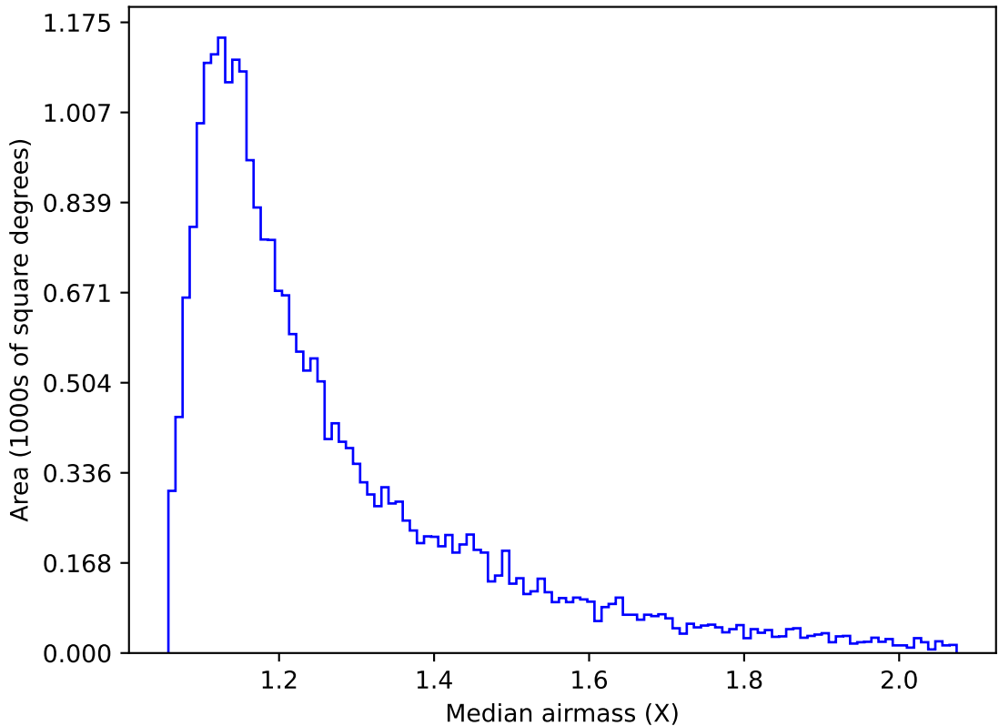
ddf_acor_sf10_lsf40_lsr10_v3.4_10yrs Yr 1 g band: Median airmass
