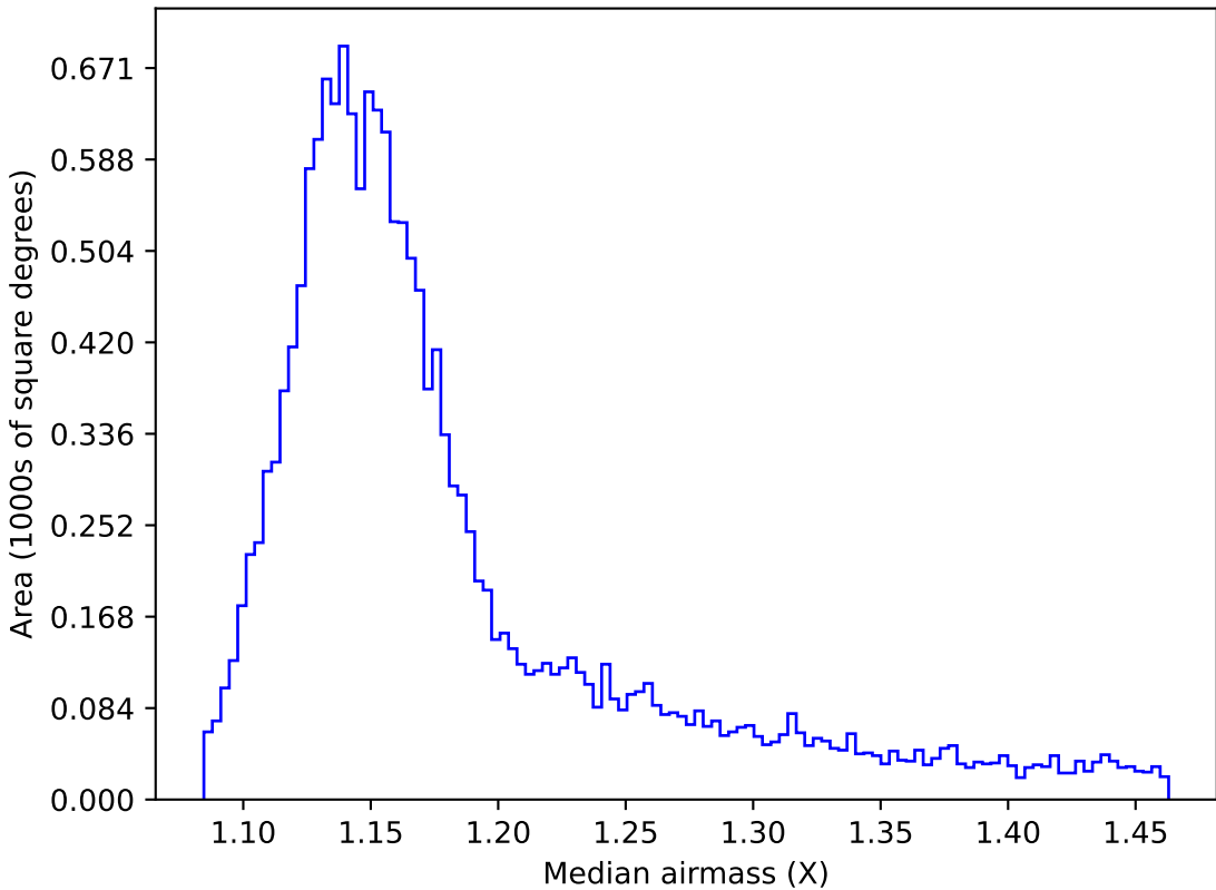
ddf_acor_sf10_lsf40_lsr10_v3.4_10yrs WFD z band: Median airmass
