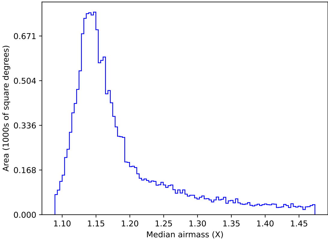
ddf_acor_sf10_ls40_lsr10_v3.4_10yrs WFD y band: Median airmass
