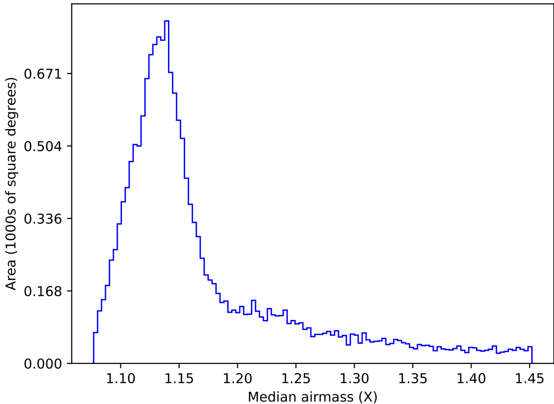
ddf_acor_sf10_lsf40_lsr10_v3.4_10yrs WFD i band: Median airmass
