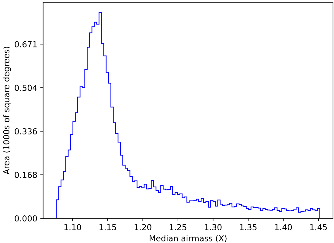
ddf_acor_sf10_lsf40_lsr10_v3.4_10yrs WFD i band: Median airmass
