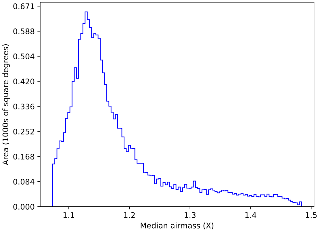
ddf_acor_sf10_lsf40_lsr10_v3.4_10yrs WFD g band: Median airmass
