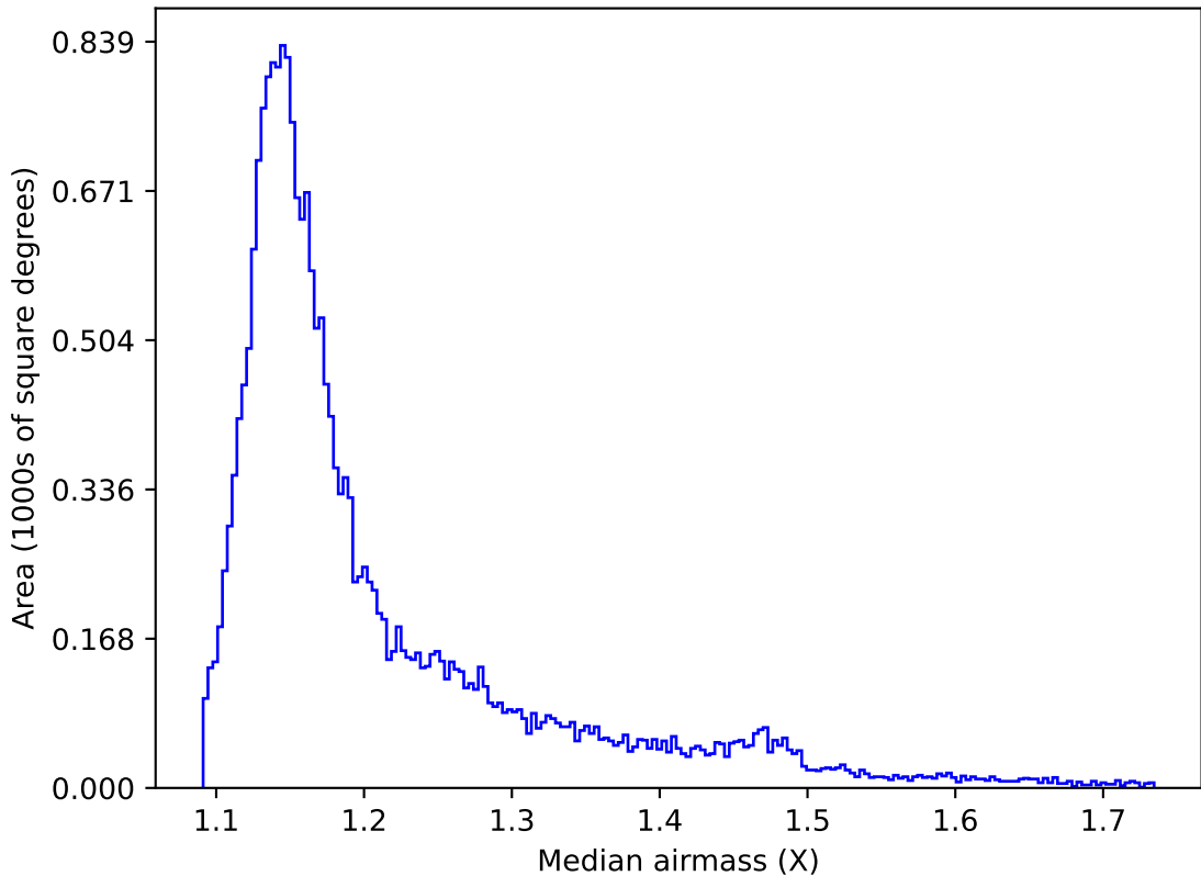
ddf_acor_sf10_lsf40_lsr10_v3.4_10yrs All sky y band: Median airmass
