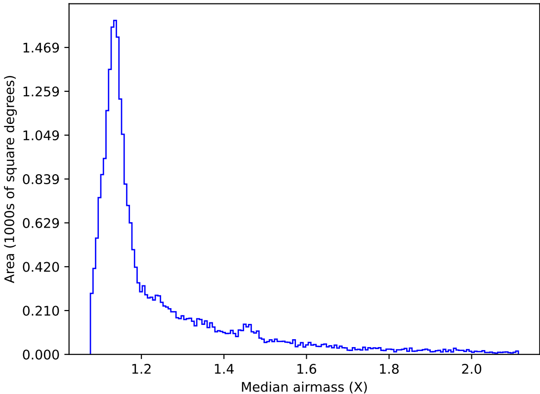
ddf_acor_sf10_lsf40_lsr10_v3.4_10yrs All sky r band: Median airmass
