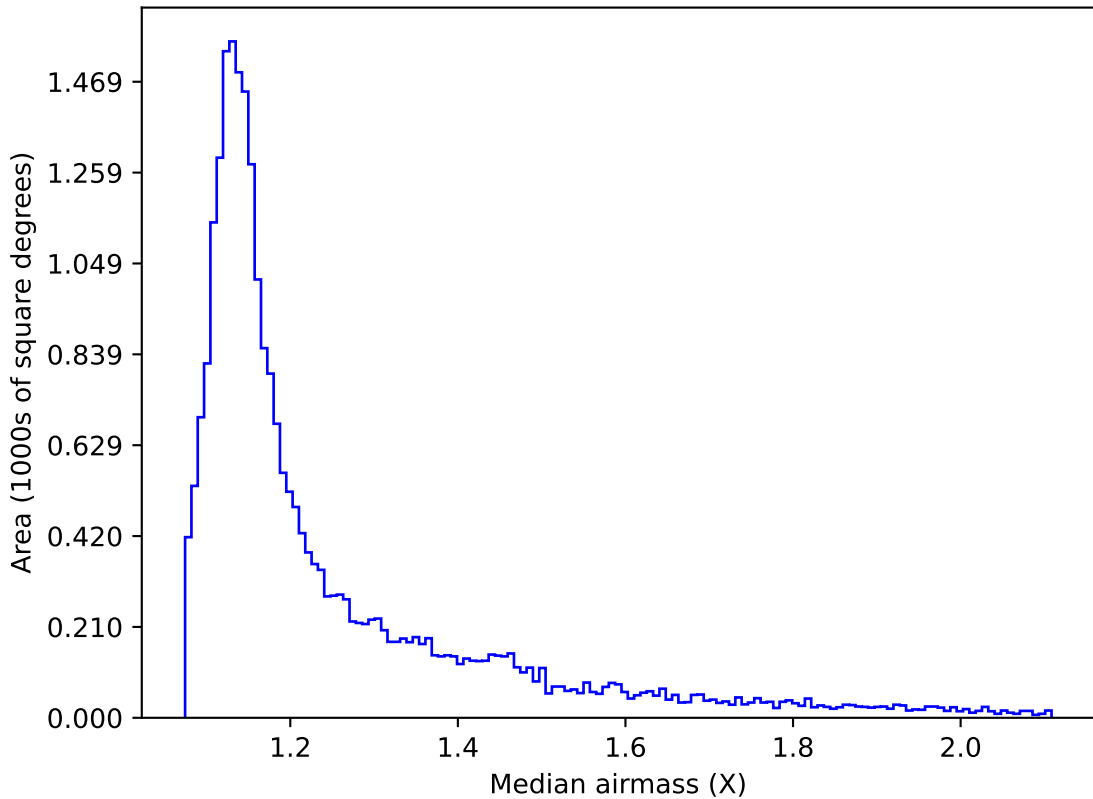
ddf_acor_sf10_lsf40_lsr10_v3.4_10yrs All sky g band: Median airmass
