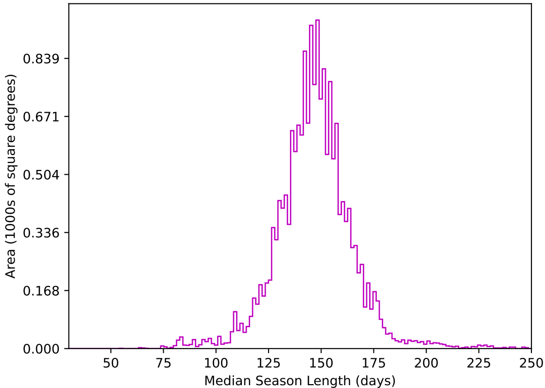
ddf_acor_sf10_ls40_lsr10_v3.4_10yrs WFD z band: Median Season Length
