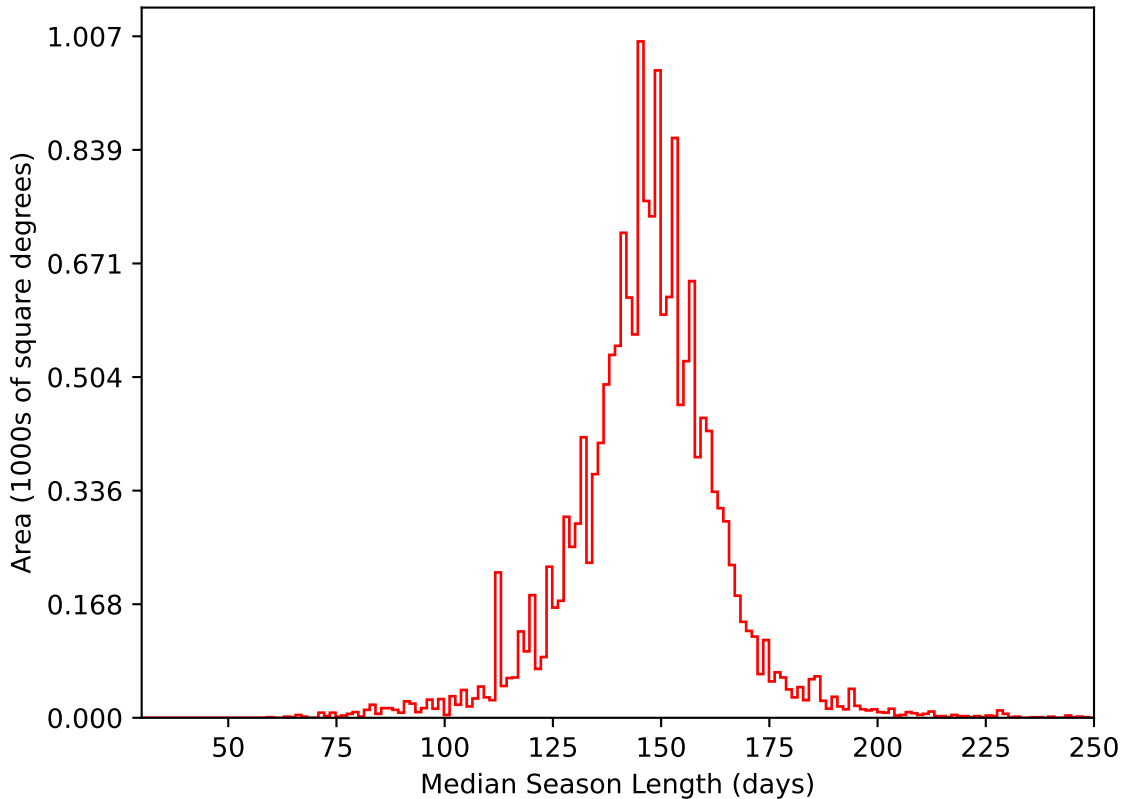
ddf_acor_sf10_lsf40_lsr10_v3.4_10yrs WFD i band: Median Season Length
