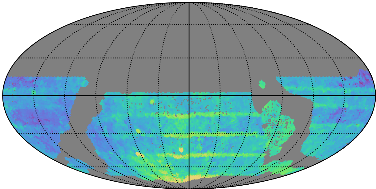
ddf_acor_sf10_lsf40_lsr10_v3.4_10yrs WFD all bands: Median Season Length
