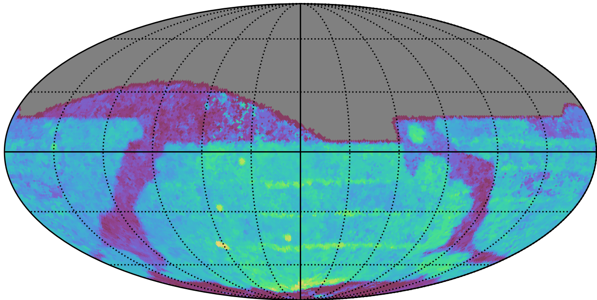
ddf_acor_sf10_lsf40_lsr10_v3.4_10yrs All sky z band: Median Season Length
