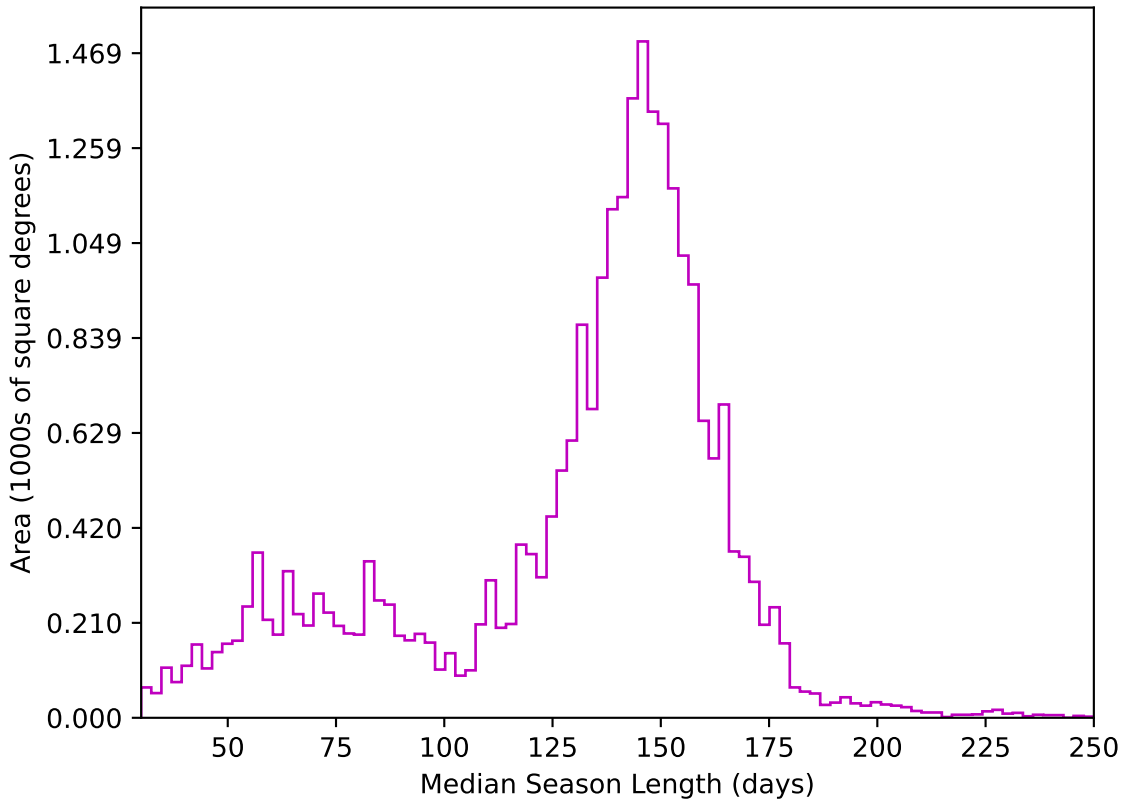
ddf_acor_sf10_lsf40_lsr10_v3.4_10yrs All sky z band: Median Season Length
