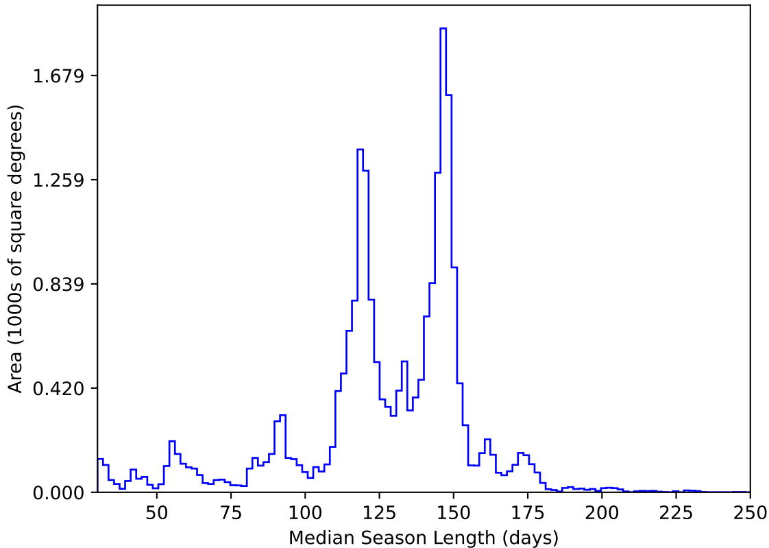
ddf_acor_sf10_lsf40_lsr10_v3.4_10yrs All sky y band: Median Season Length
