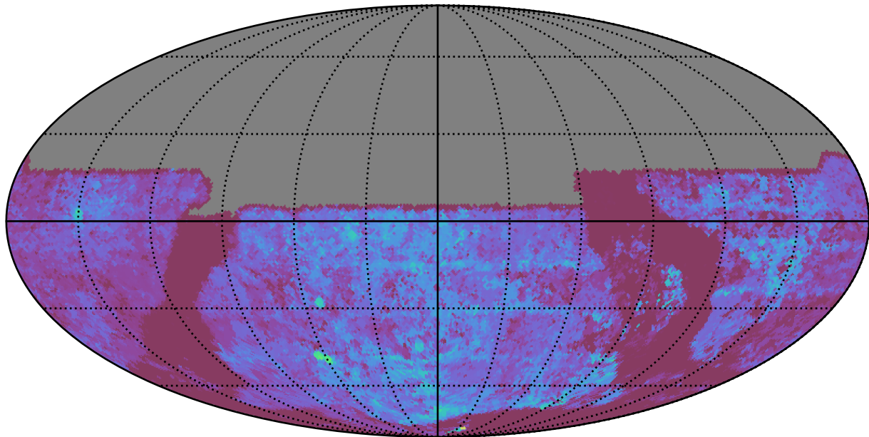
ddf_acor_sf10_lsf40_lsr10_v3.4_10yrs All sky u band: Median Season Length
