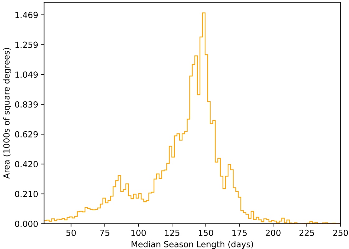
ddf_acor_sf10_lsf40_lsr10_v3.4_10yrs All sky r band: Median Season Length
