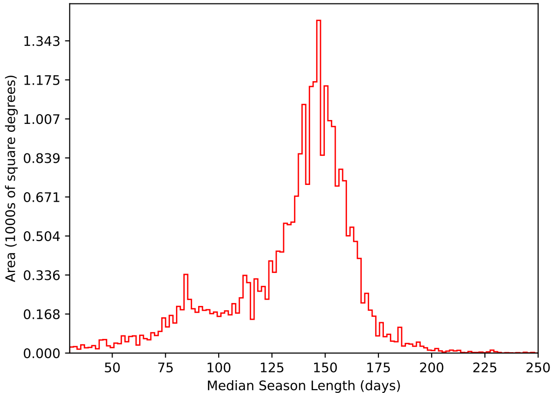
ddf_acor_sf10_lsf40_lsr10_v3.4_10yrs All sky i band: Median Season Length
