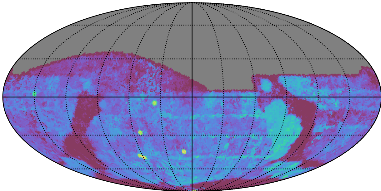
ddf_acor_sf10_lsf40_lsr10_v3.4_10yrs All sky g band: Median Season Length
