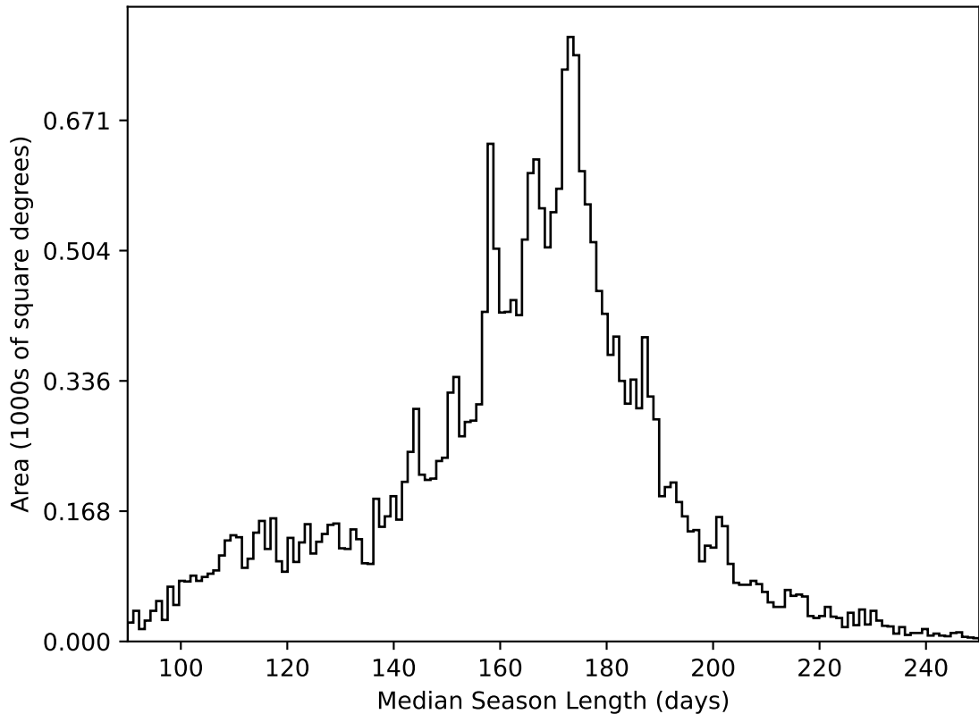
ddf_acor_sf10_lsf40_lsr10_v3.4_10yrs All sky all bands: Median Season Length
