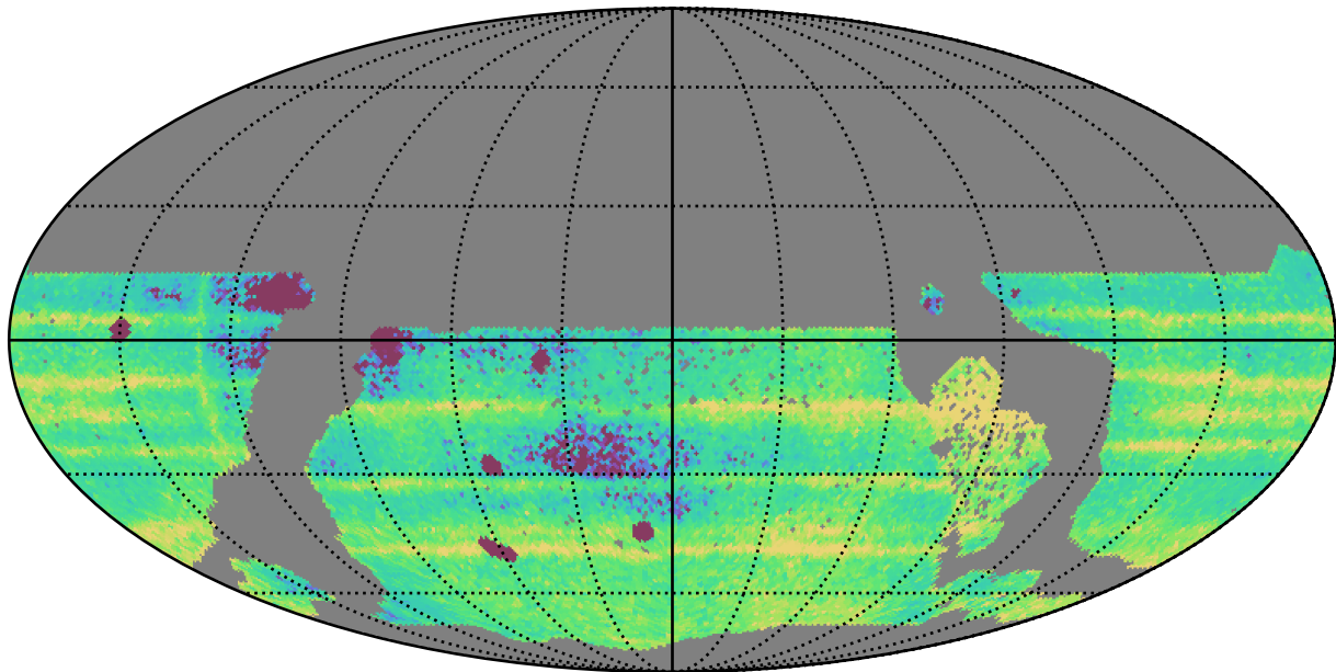
ddf_acor_sf10_lsf40_lsr10_v3.4_10yrs WFD: Median Intra-Night Gap
