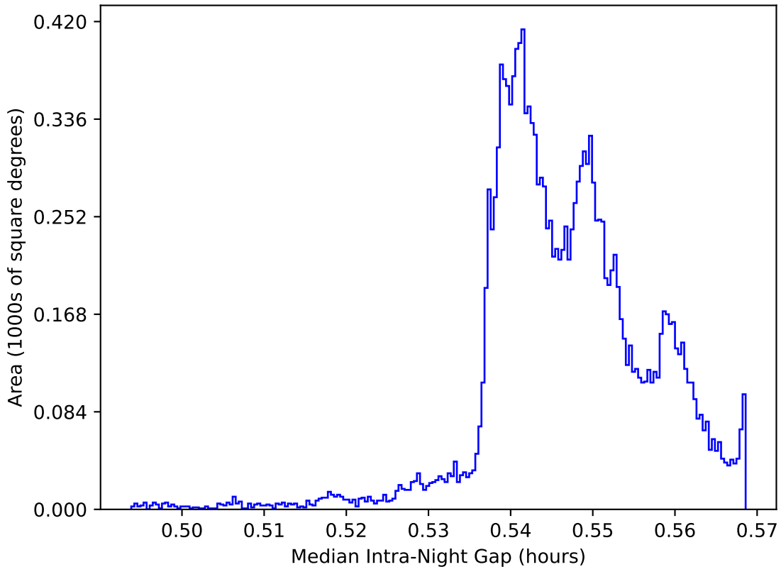
ddf_acor_sf10_ls40_lsr10_v3.4_10yrs WFD: Median Intra-Night Gap
