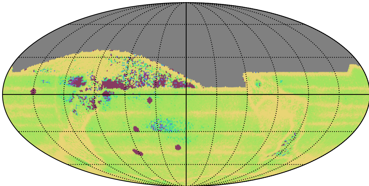
ddf_acor_sf10_lsf40_lsr10_v3.4_10yrs All sky: Median Intra-Night Gap
