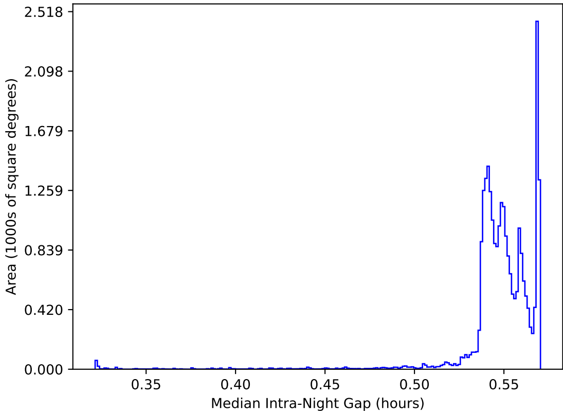
ddf_acor_sf10_lsf40_lsr10_v3.4_10yrs All sky: Median Intra-Night Gap
