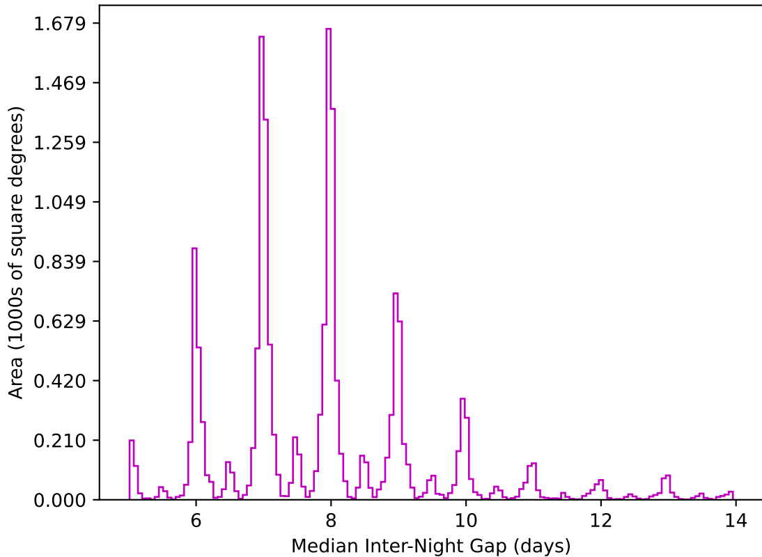
ddf_acor_sf10_lsf40_lsr10_v3.4_10yrs WFD z band: Median Inter-Night Gap
