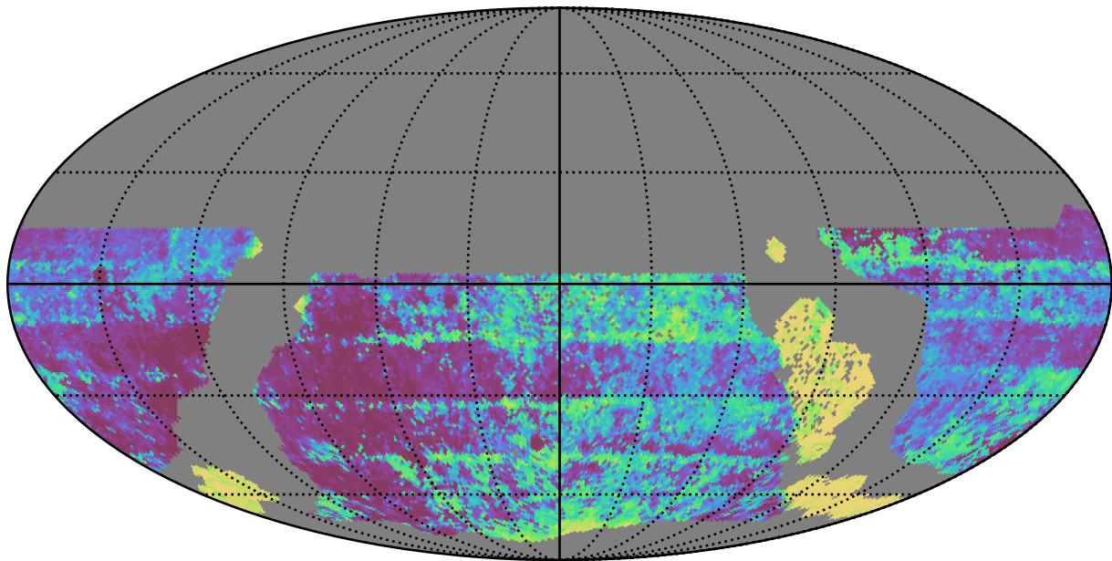
ddf_acor_sf10_lsf40_lsr10_v3.4_10yrs WFD y band: Median Inter-Night Gap
