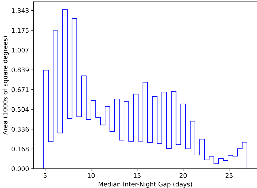
ddf_acor_sf10_lsf40_lsr10_v3.4_10yrs WFD y band: Median Inter-Night Gap
