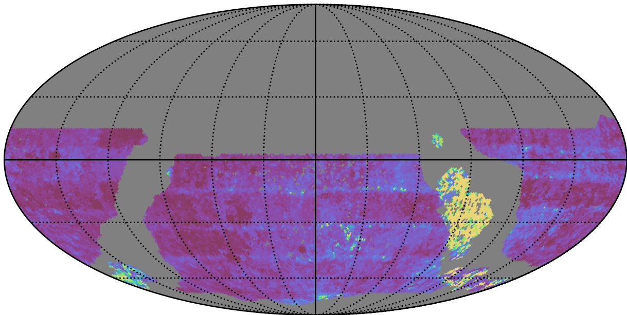
ddf_acor_sf10_lsf40_lsr10_v3.4_10yrs WFD u band: Median Inter-Night Gap
