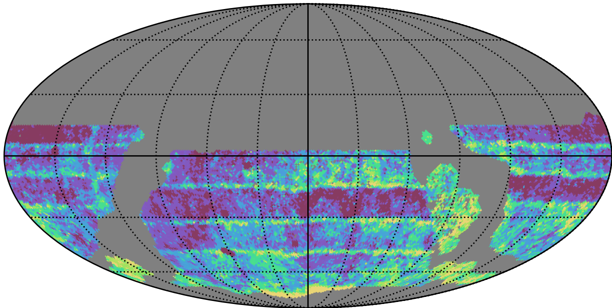
ddf_acor_sf10_lsf40_lsr10_v3.4_10yrs WFD r band: Median Inter-Night Gap
