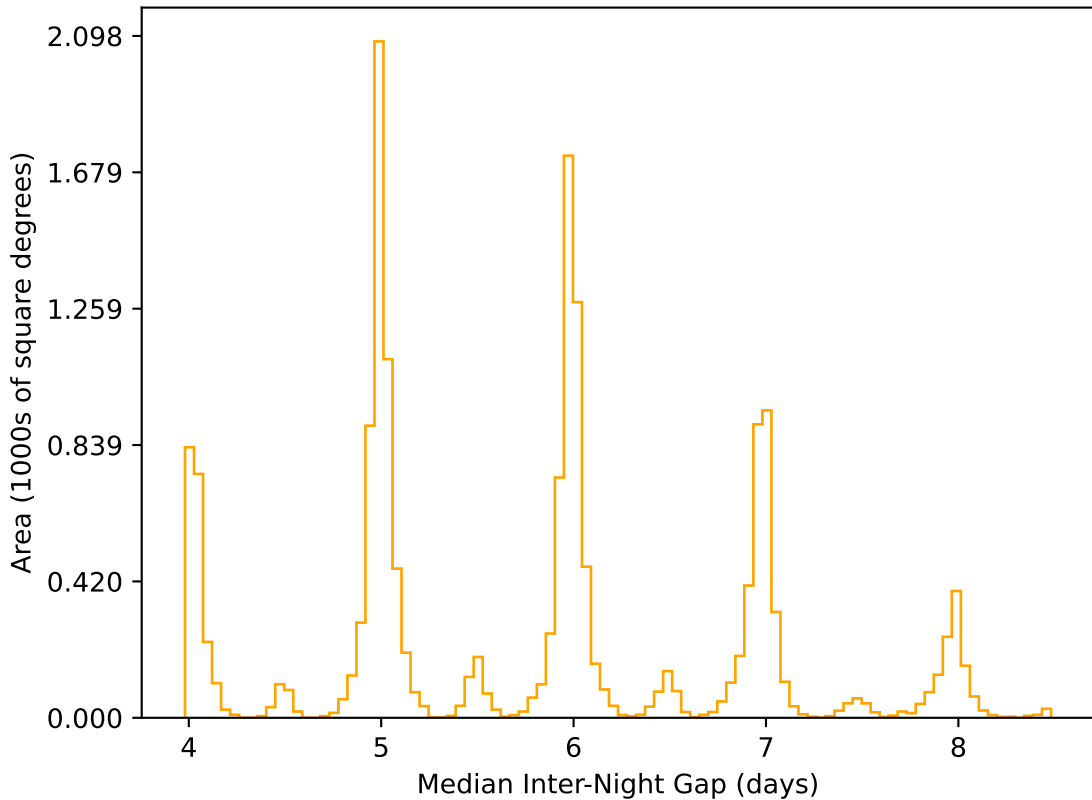
ddf_acor_sf10_lsf40_lsr10_v3.4_10yrs WFD r band: Median Inter-Night Gap
