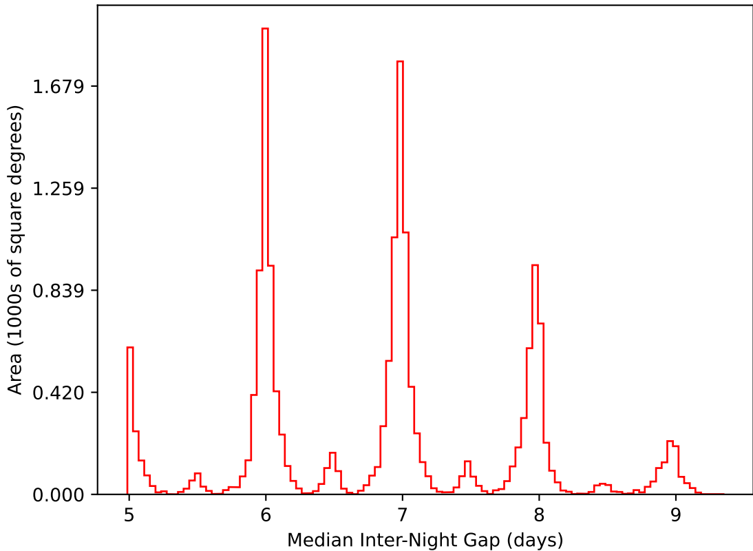
ddf_acor_sf10_lsf40_lsr10_v3.4_10yrs WFD i band: Median Inter-Night Gap
