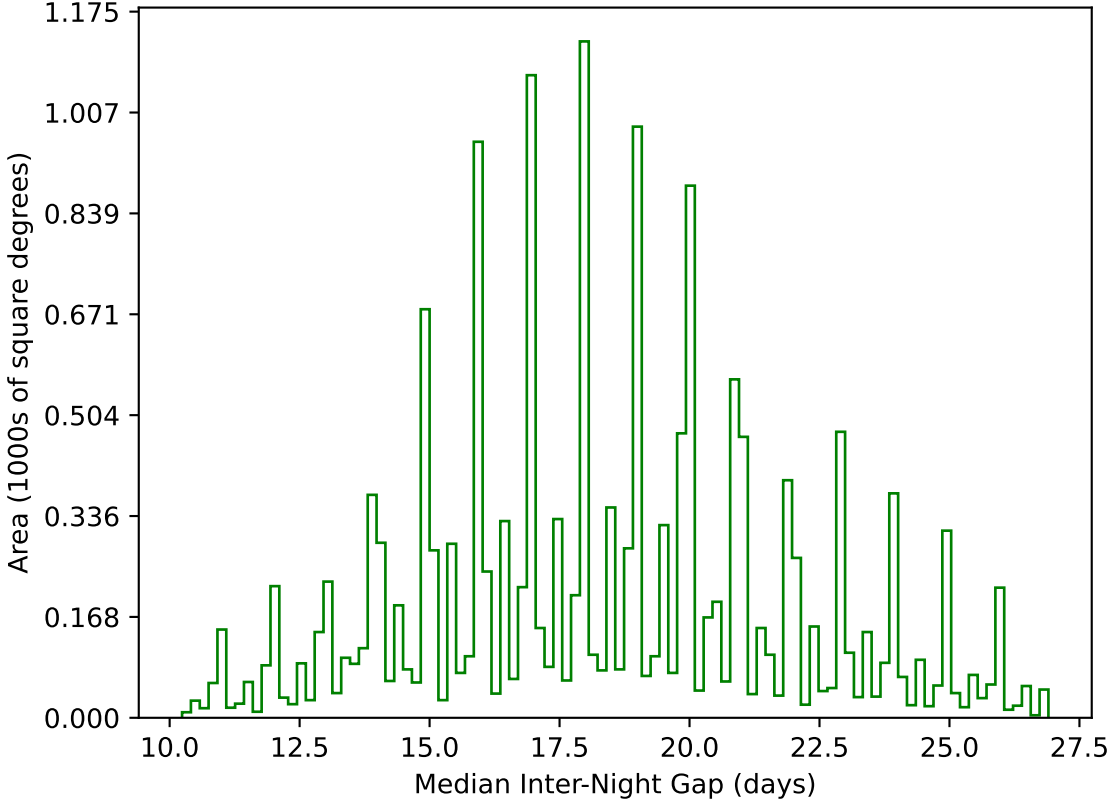
ddf_acor_sf10_lsf40_lsr10_v3.4_10yrs WFD g band: Median Inter-Night Gap
