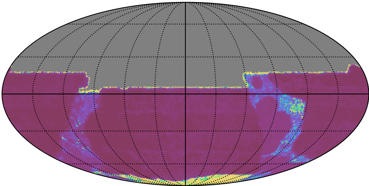
ddf_acor_sf10_lsf40_lsr10_v3.4_10yrs All sky y band: Median Inter-Night Gap
