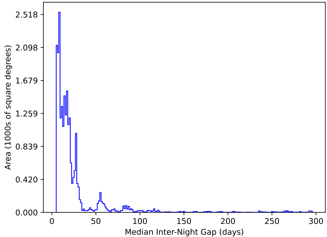
ddf_acor_sf10_lsf40_lsr10_v3.4_10yrs All sky y band: Median Inter-Night Gap
