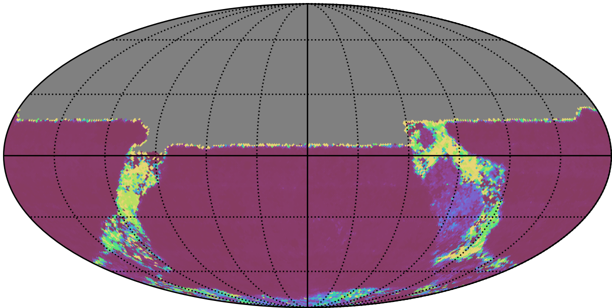
ddf_acor_sf10_lsf40_lsr10_v3.4_10yrs All sky u band: Median Inter-Night Gap
