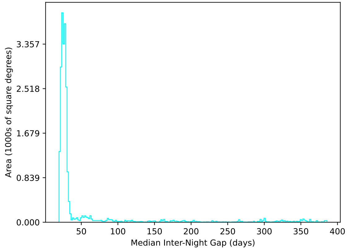
ddf_acor_sf10_lsf40_lsr10_v3.4_10yrs All sky u band: Median Inter-Night Gap
